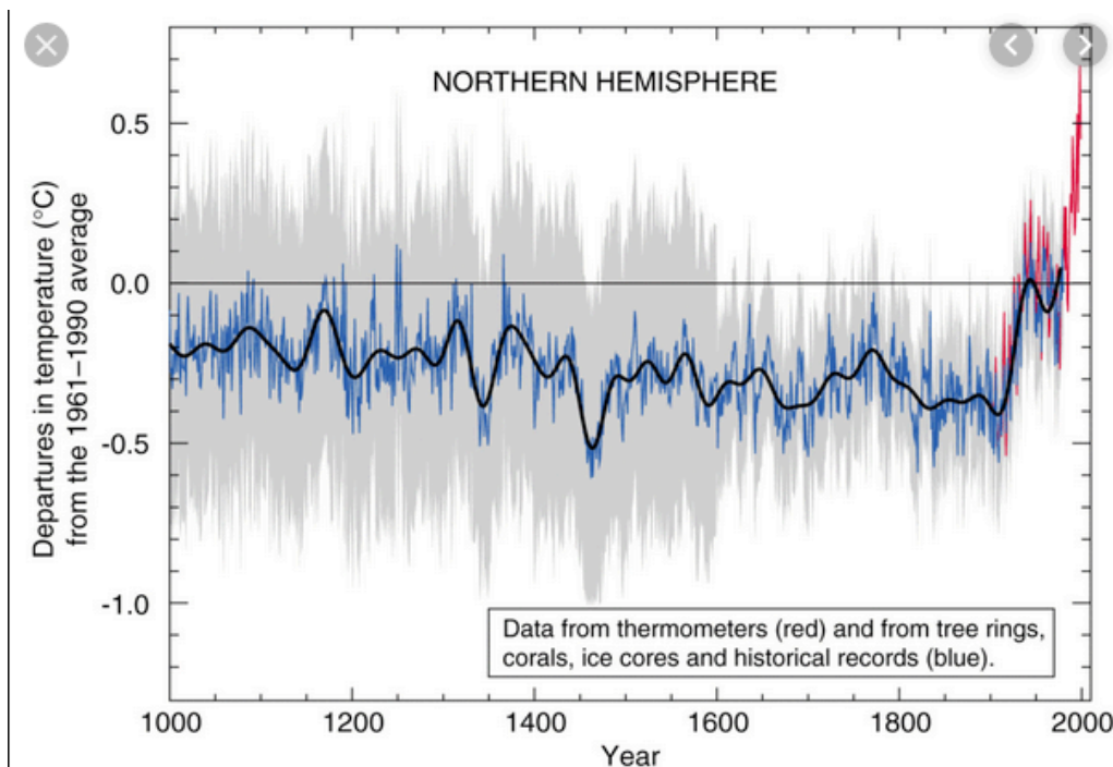
Figure 14. Michael Mann's Hockey Stick
